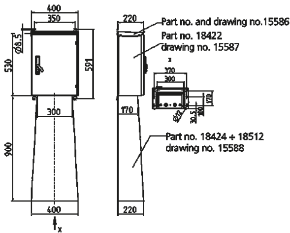
Drawing 1 MB 437
