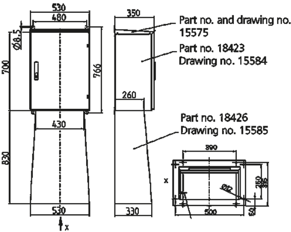
Drawing 1 MB 439
