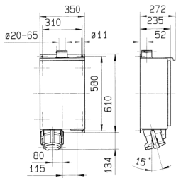
Drawing 1 MB 387 Dim. in mm
