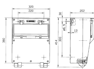
Drawing 5 MB 41 Dim. in mm
