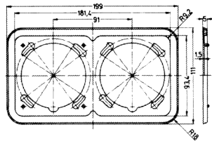
Drawing 1 MB 364 Dim. in mm
