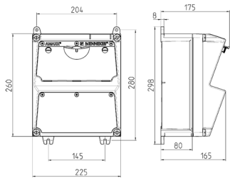
Drawing 1 MB 521
