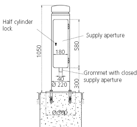
Drawing 1 MB 443 Dim. in mm
