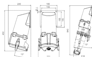
Drawing 1 MB 637 Dim. in mm
