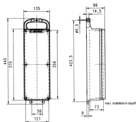
Drawing 5 MB 44
