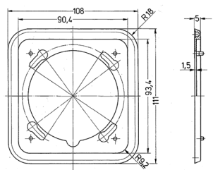
Drawing 1 MB 363 Dim. in mm
