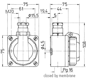
Drawing 1 MB 347 Dim. in mm
