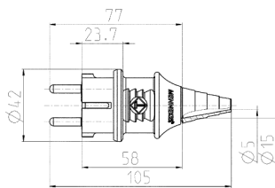
Drawing 2 MB 139 Dim. in mm
