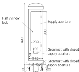
Drawing 1 MB 445 Dim. in mm
