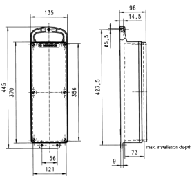
Drawing 5 MB 44 Dim. in mm
