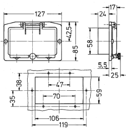
Drawing 6 MB 2 Dim. in mm
