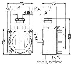
Drawing 1 MB 347 Dim. in mm
